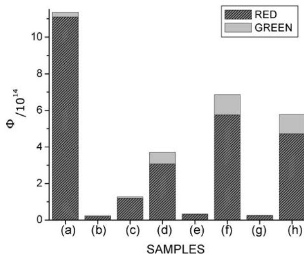
Fig. 5 Comparison of the number of photons ( \Phi ) of the Er, Yb samples, estimated from emission spectra recorded at room temperature and excitation at 10,212\text{ cm}^{-1} and 10,240\text{ cm}^{-1} for oxysulfide and oxide ones respectively for an incident power of 100 mW (unfocused beam)
